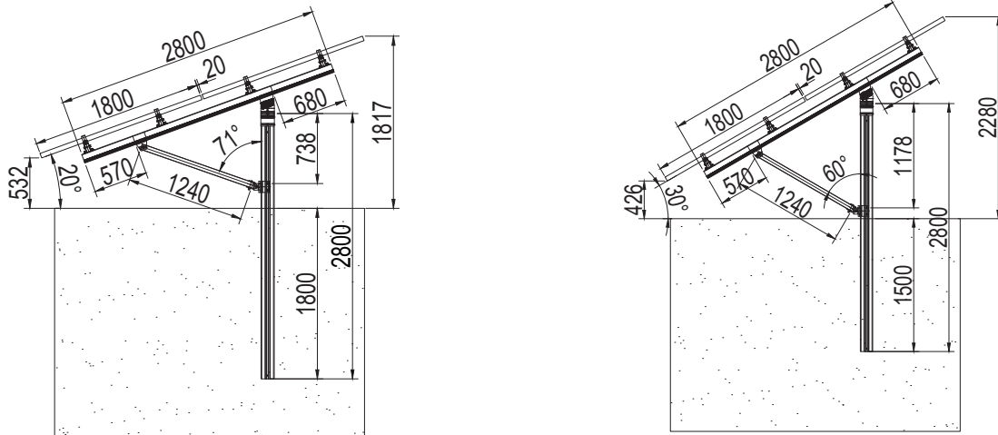
Side view drawings of support for panels up to 1800 x 1400 mm
