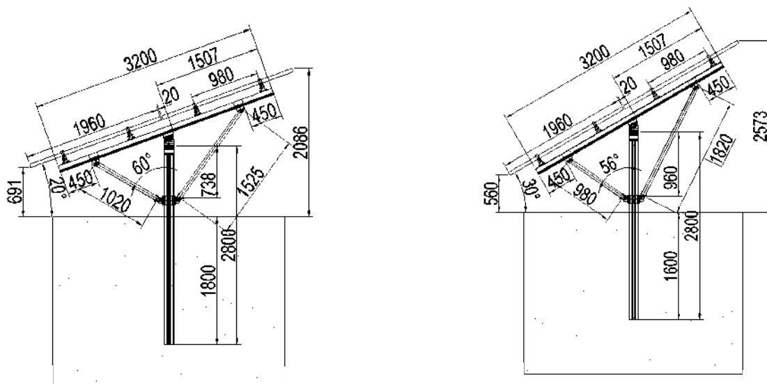
Side view drawings of support for panels up to 2000 x 1400mm
